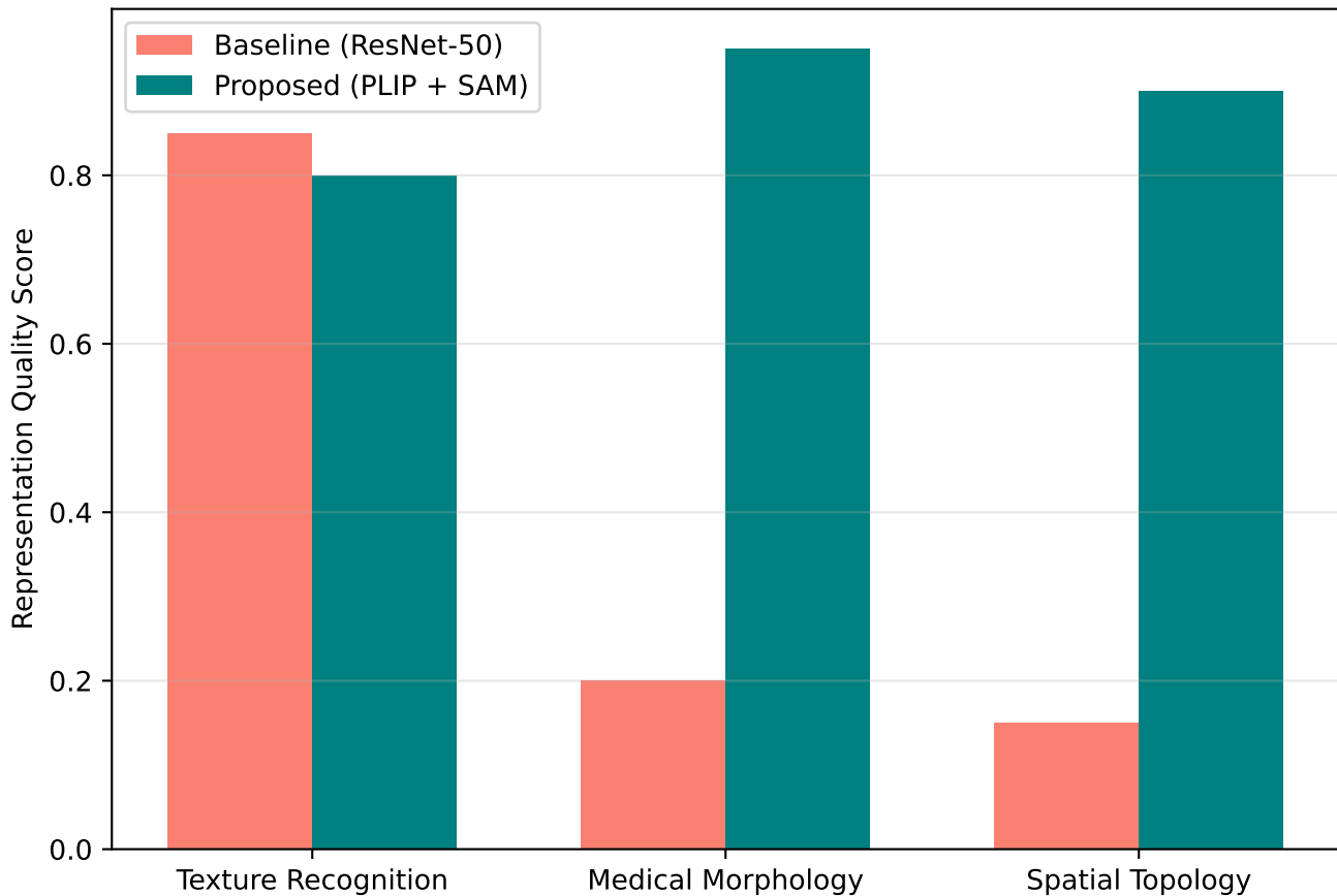
Gap 2 Analysis: Domain-Specific Embeddings
